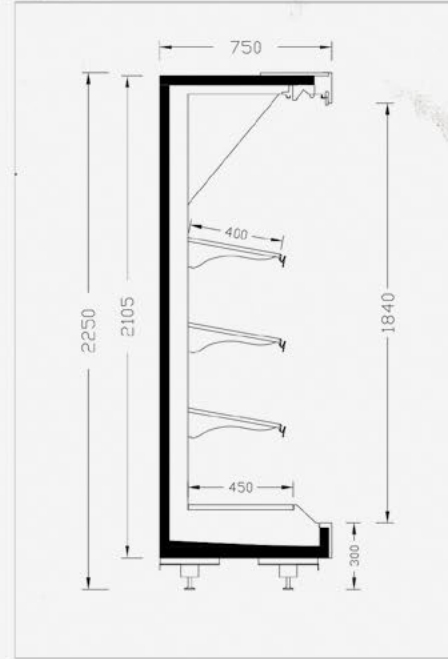
ELITE GG 75-225
