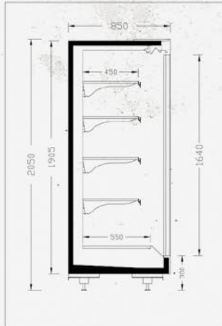
ELITE SD 85-205
