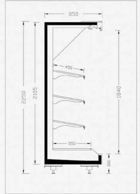
ELITE GG 85-225
