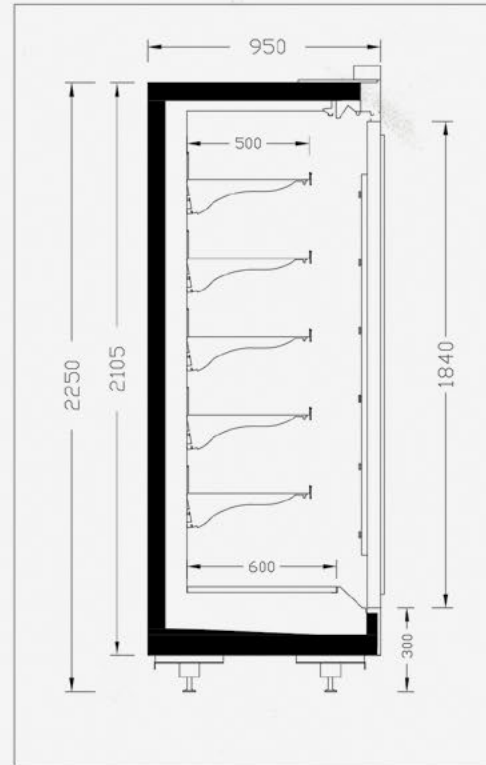
INVERNO FREEZER 95-225
