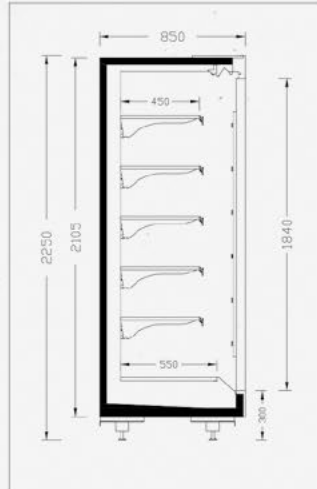
ELITE HD 85-225
