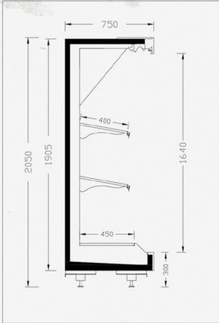
ELITE GG 75-205
