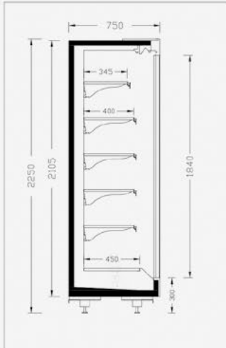
ELITE SD 75-225
