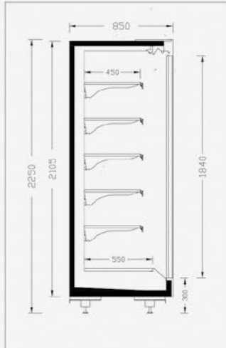
ELITE SD 85-225
