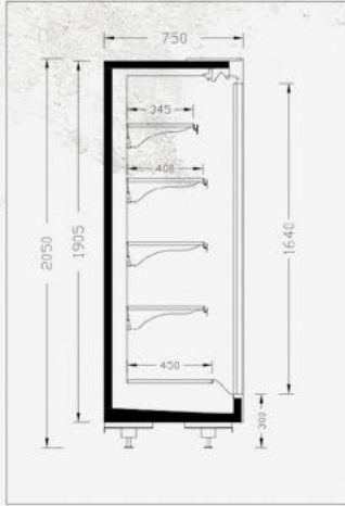
ELITE SD 75-205
