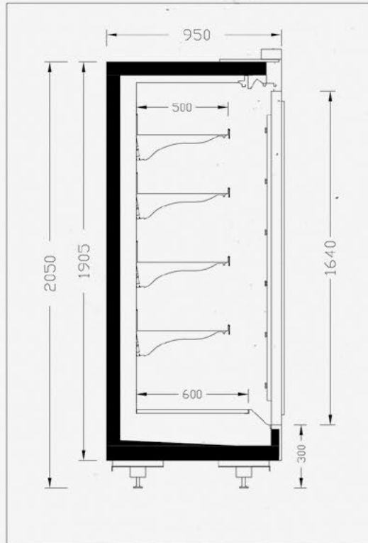
INVERNO FREEZER 95-205
