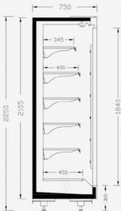
ELITE HD 75-225
