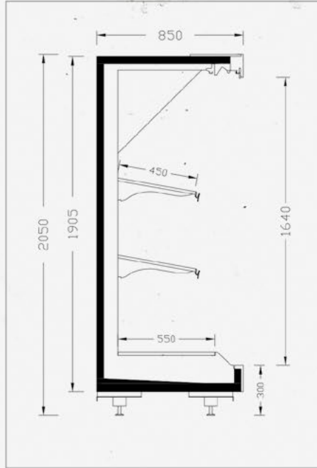
ELITE GG 85-205
